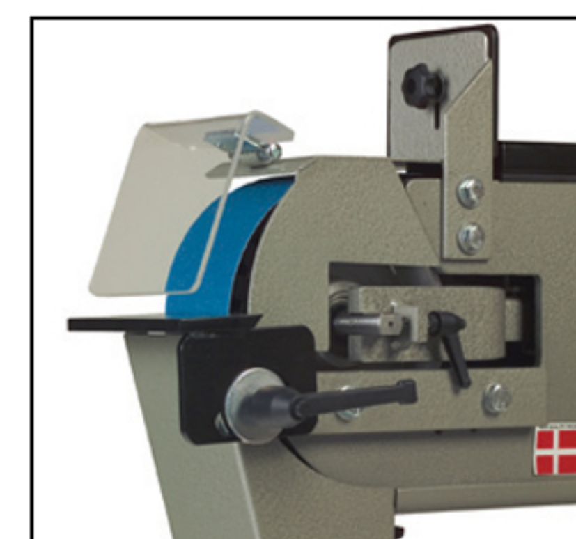
CONTACT WHEEL FOR RAPID STOCK REMOVAL
