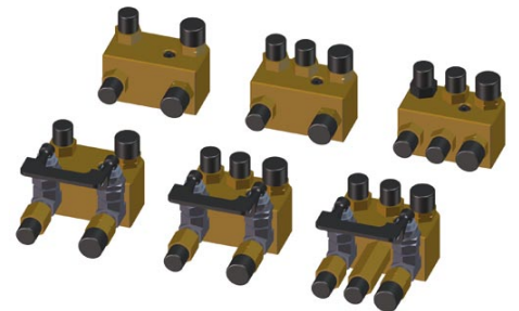
UCW-0475-59-00-00-0 Precise Machine Torch Holder φ 30mm (1.18")
