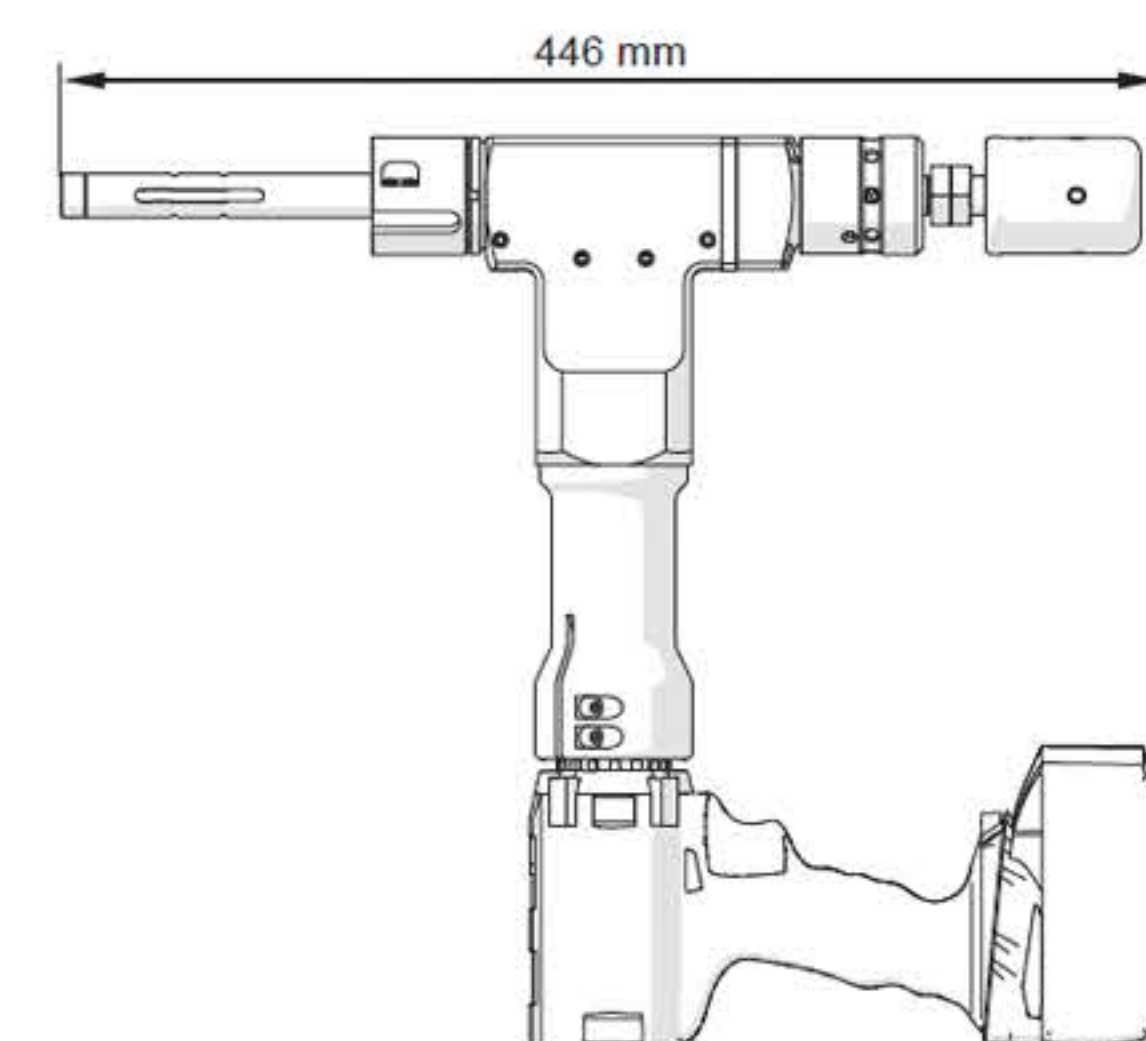
PB2 with battery motor
