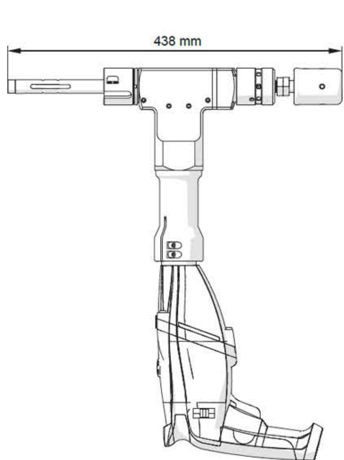
PB2 with electric motor
