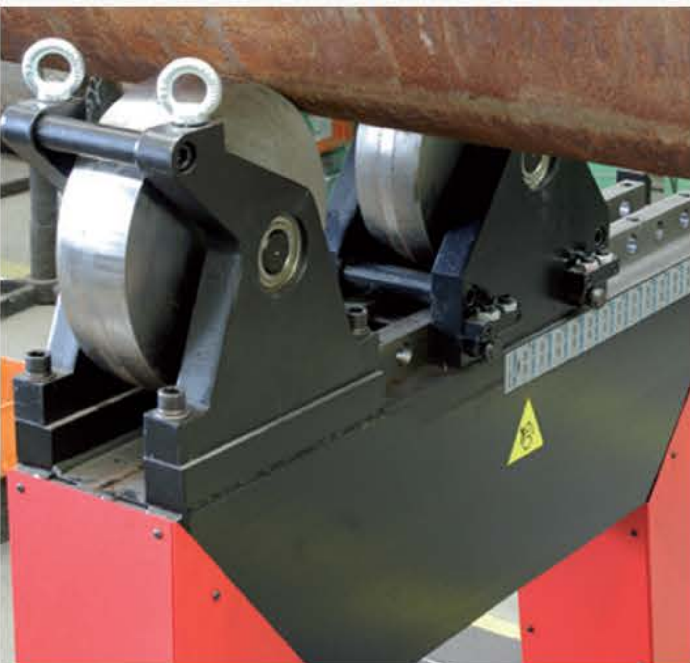
HEAVY-DUTY ADJUSTABLE PIPE SUPPORT (Ø 200-1000 MM)
