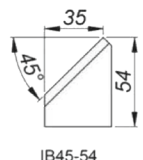
45° Internal Beveling Tool Bit, Height 54 mm [IB45/54] Product Code: PB10-IB45/54
