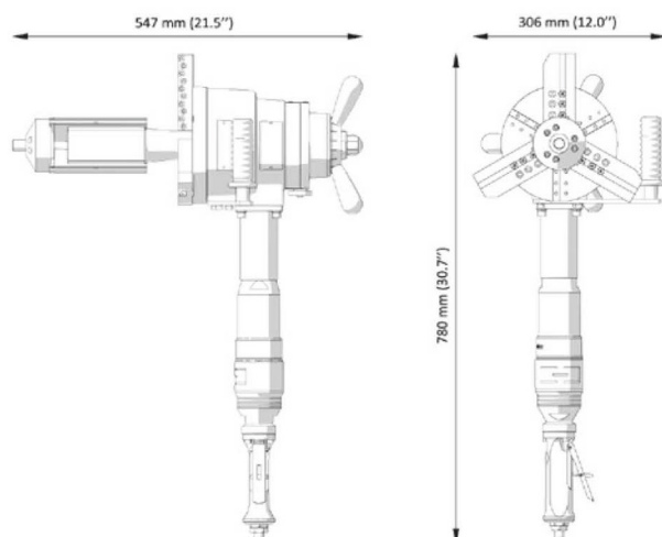
PB-14 E with Electric Motor
