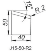
15° J-Beveling Tool Bit, Height 50 mm, Radius 2mm [J15/50/R2] Product Code: PB10-J15/50/22
