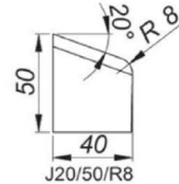
20° J-Beveling Tool Bit, Height 50 mm, Radius 8mm [J20/50/R8] Product Code: PB10-J20/50/R8
