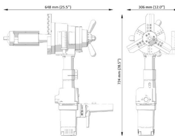
PB-14 A with Pneumatic Motor
